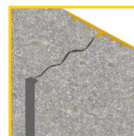
Crack Inducing Waterstop Method
